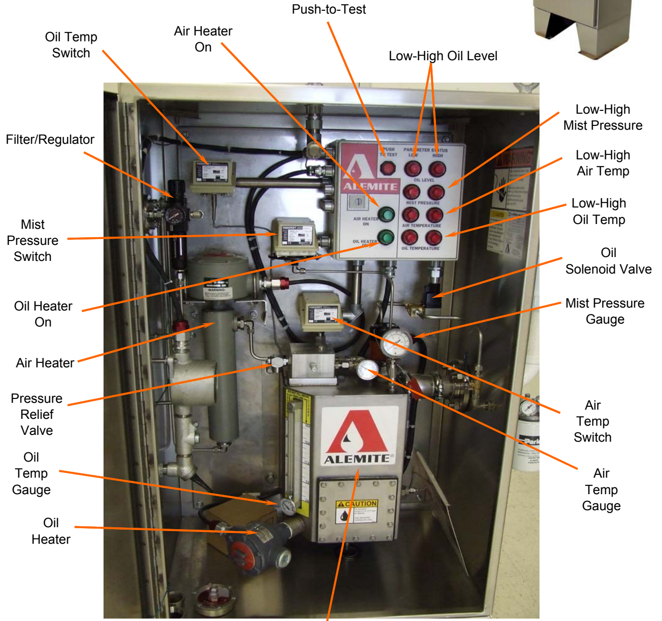
5-Gal SS Oil Reservoir w/ Level Gauge & Thermometer
